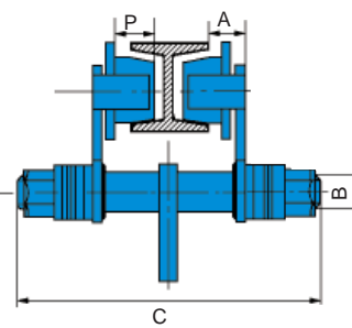
Push trolley
